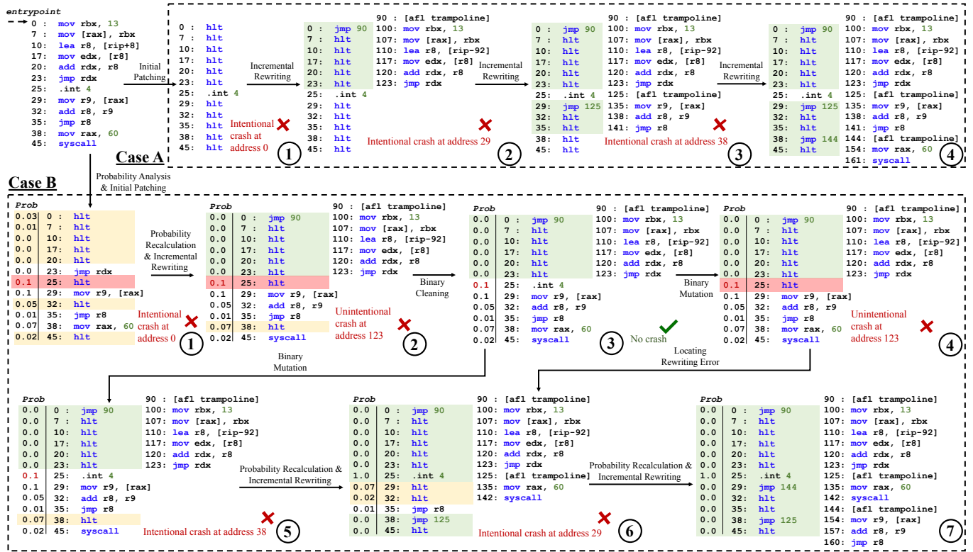
Fig. 4: How STOCHFUEZ handles the motivation example
